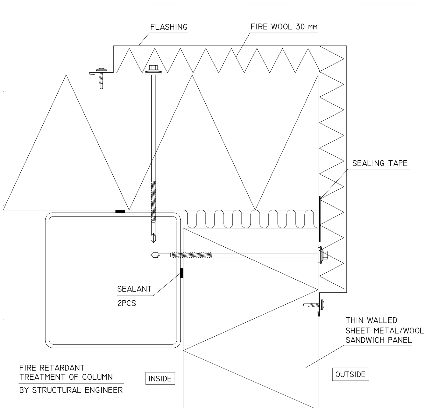
FIRE DETAIL EI90-EI240
