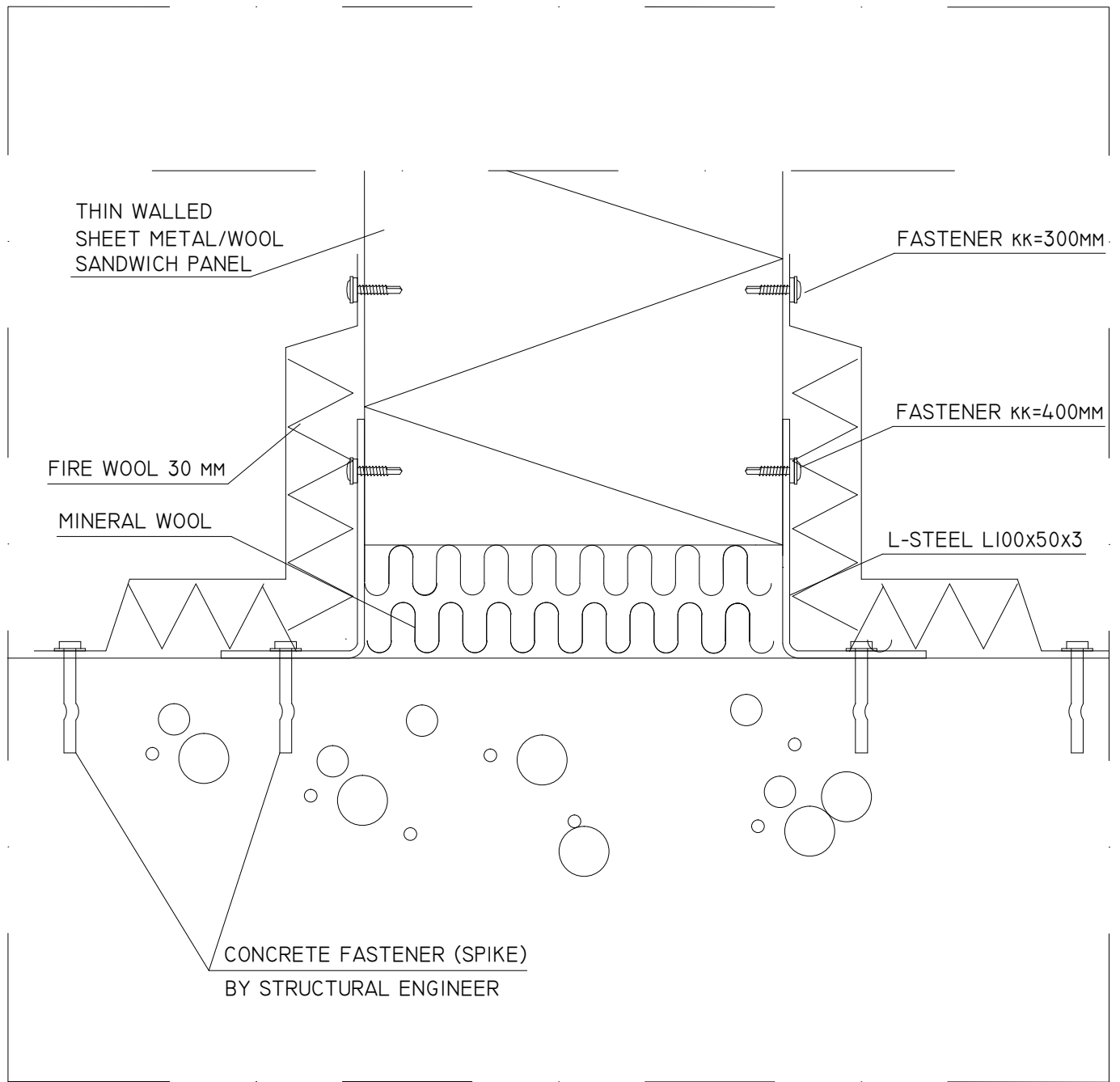
FIRE DETAIL EI90-EI240
