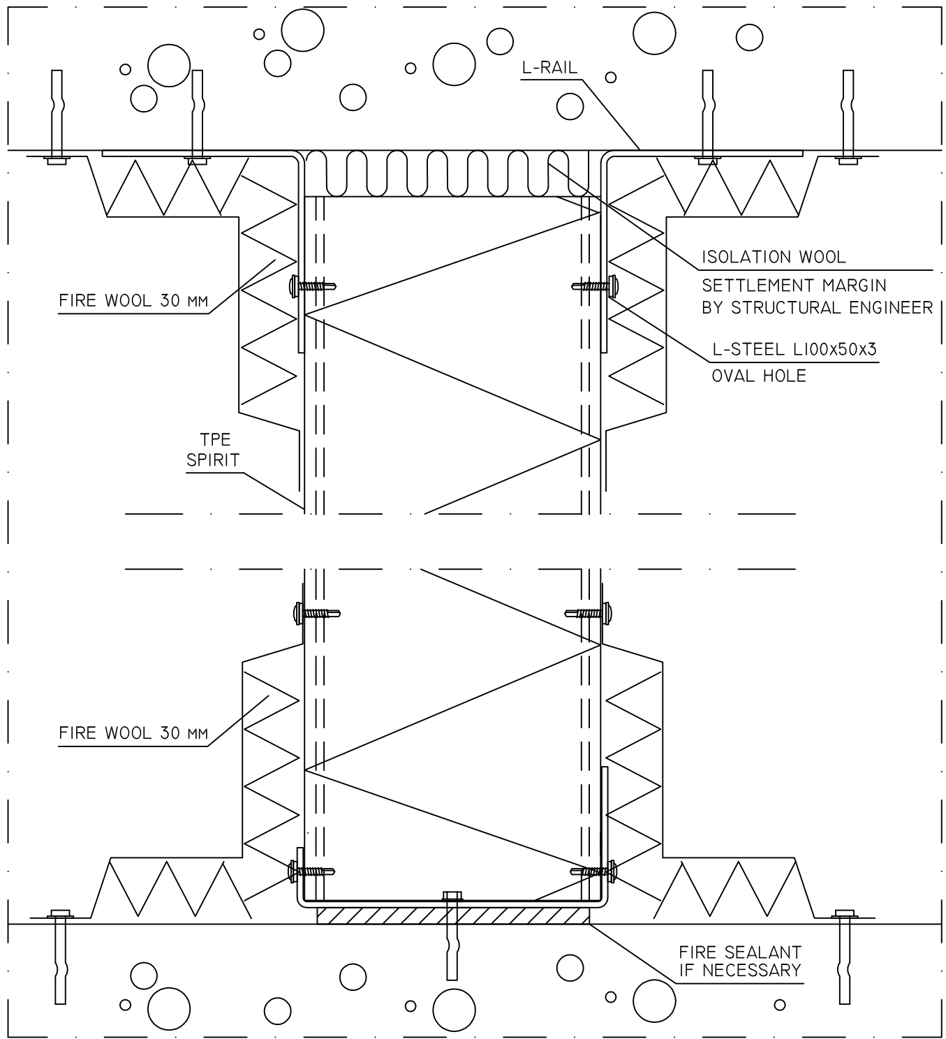
FIRE DETAIL EI90-EI240
